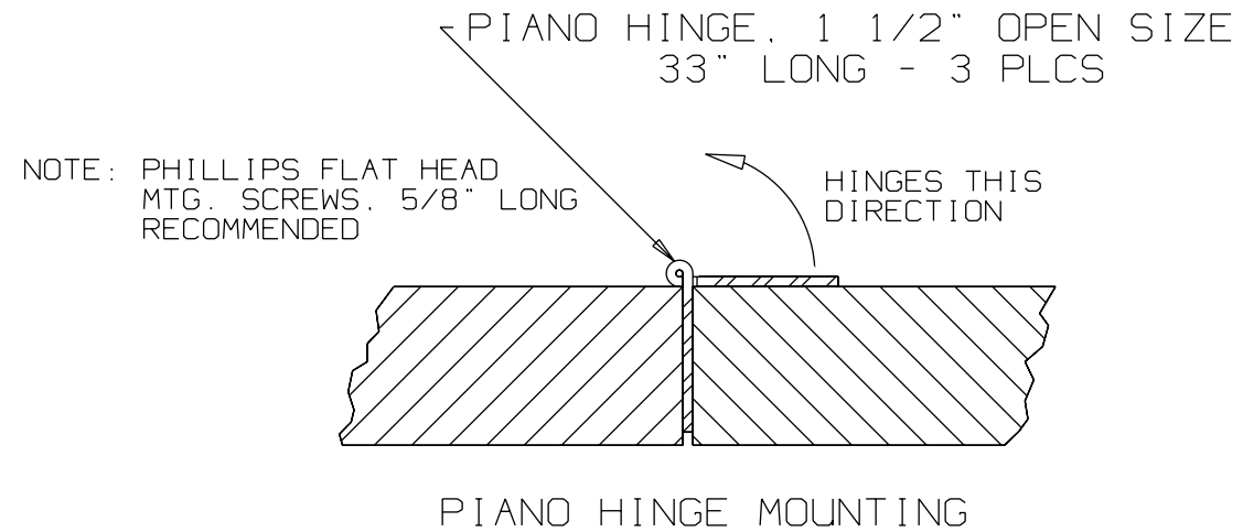
DETAIL F
